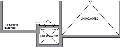
BASEMENT & OPT. FINISHED BASEMENT ELEVATION B
