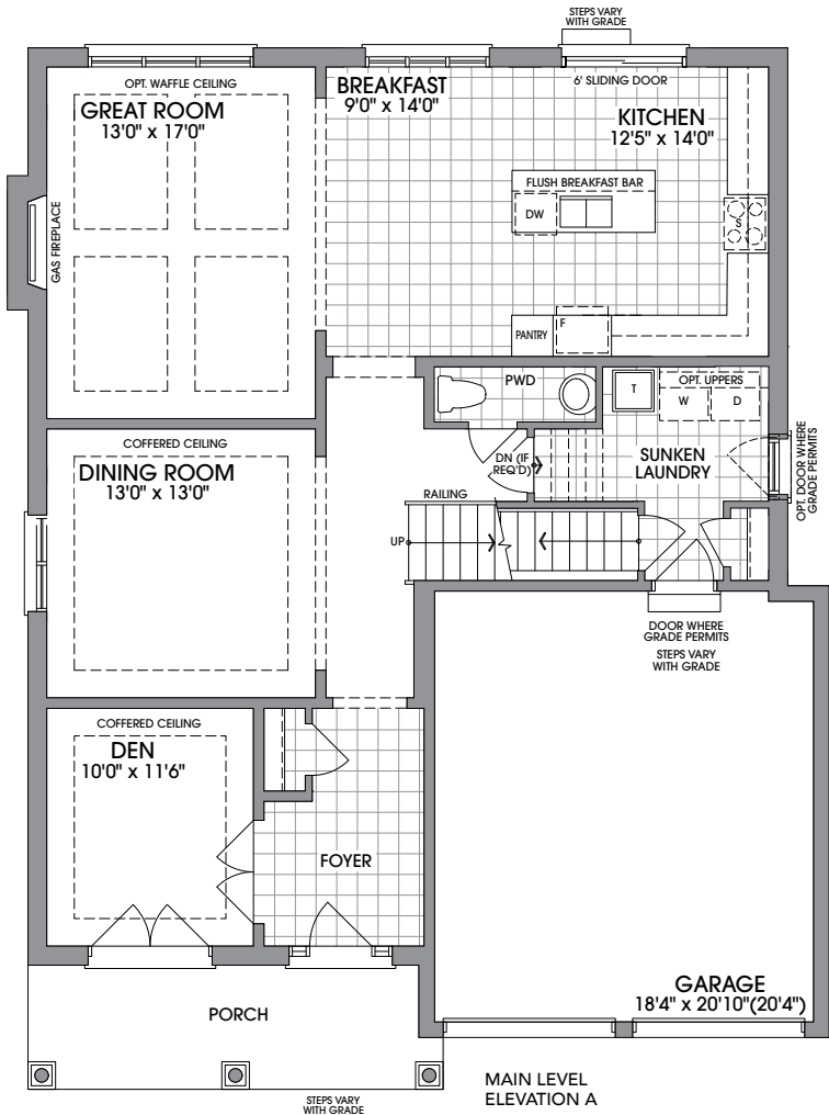
MAIN LEVEL ELEVATION A
