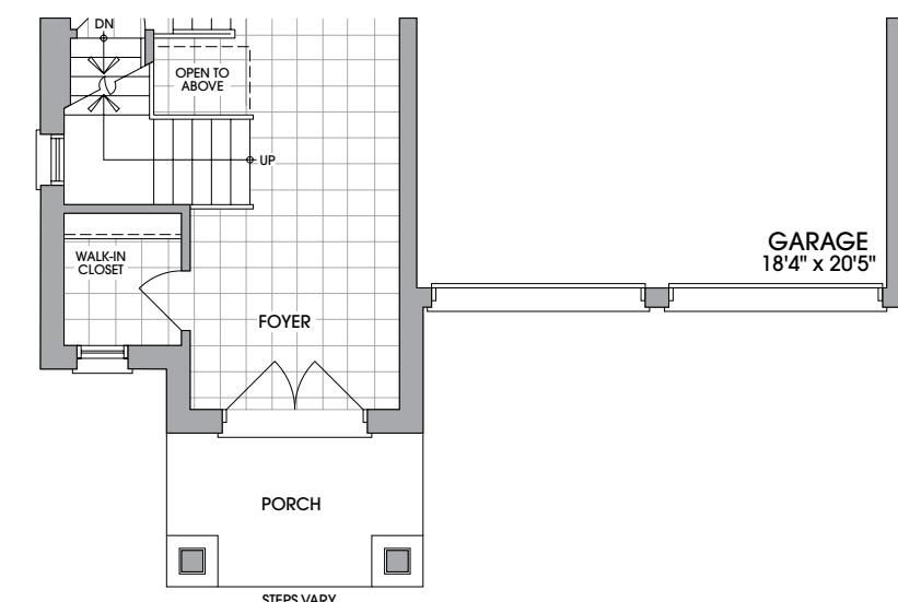
MAIN LEVEL ELEVATION B
