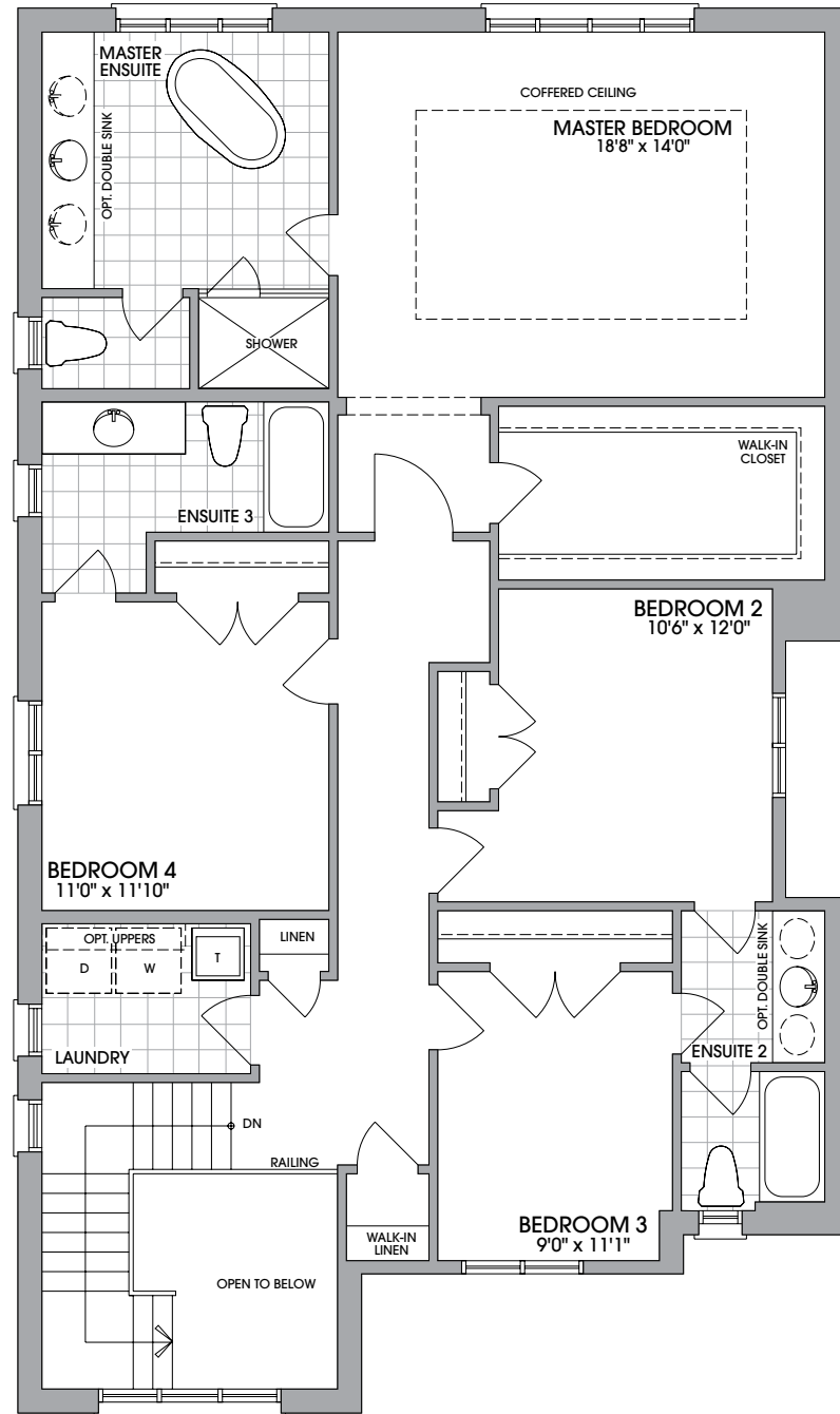
UPPER LEVEL ELEVATION A
