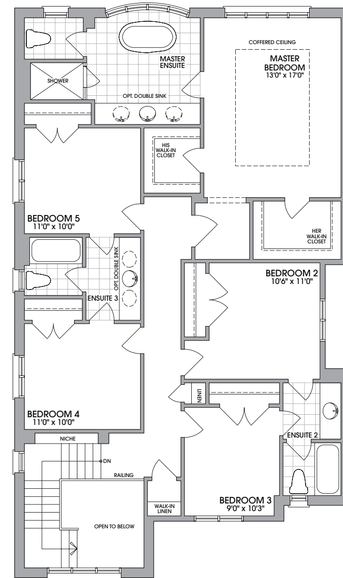
UPPER LEVEL OPT. 5 BEDROOM ELEVATION A
